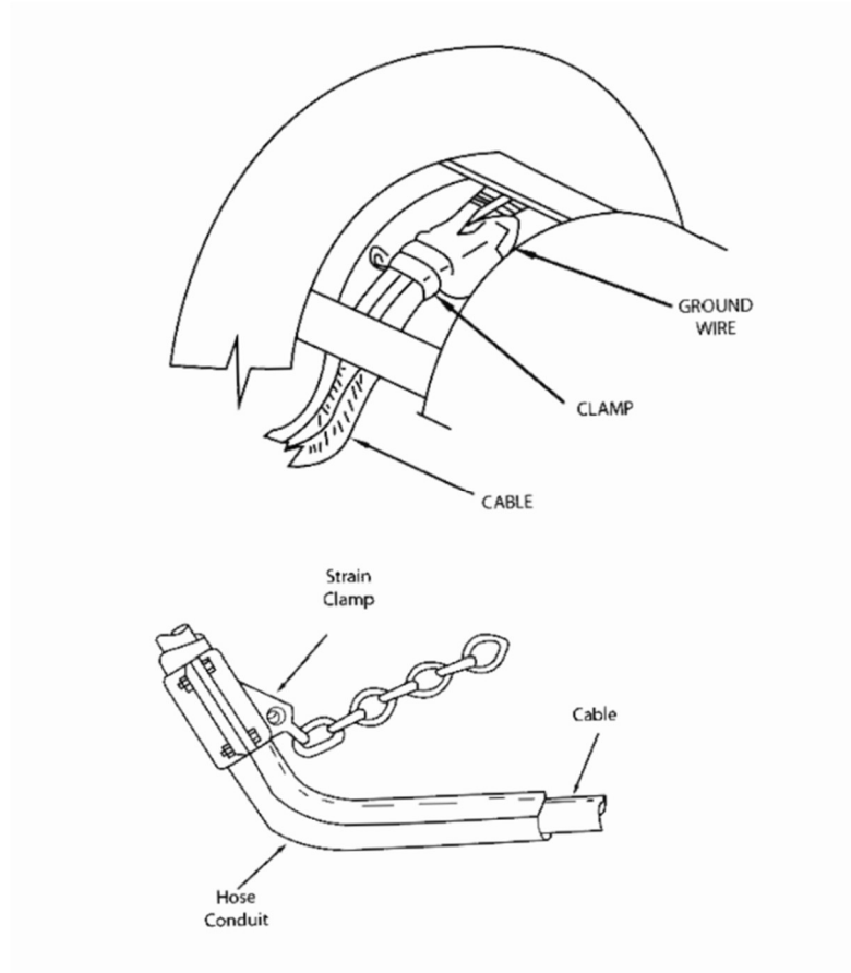
2.8: Strain connection on cables
