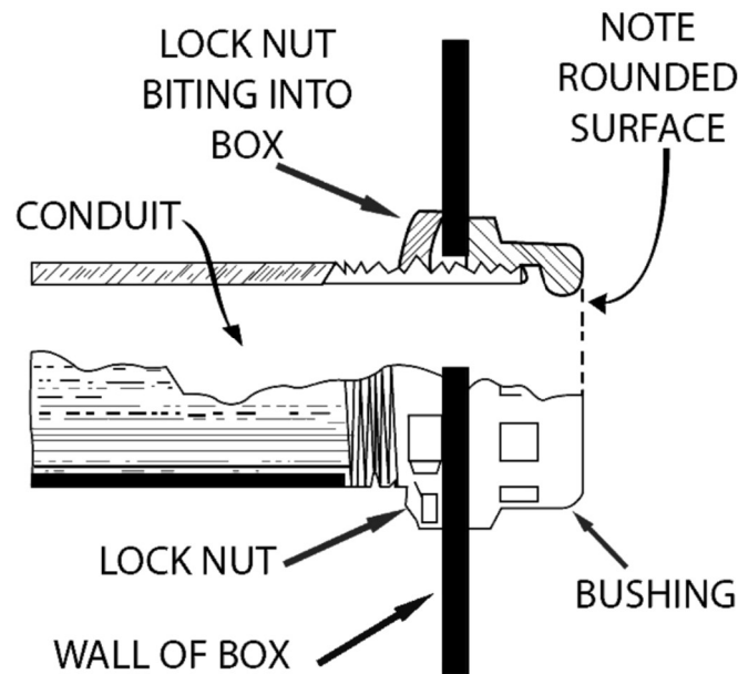
2.7: Insulated bushing
