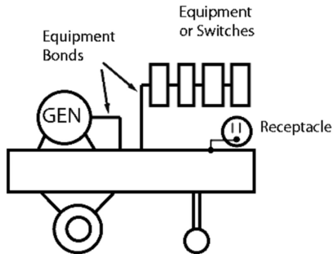
2.15: Vehicle mounted generator
