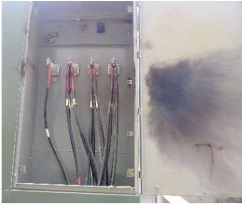
2.23: Damage upon transformer due to arc flash accident
