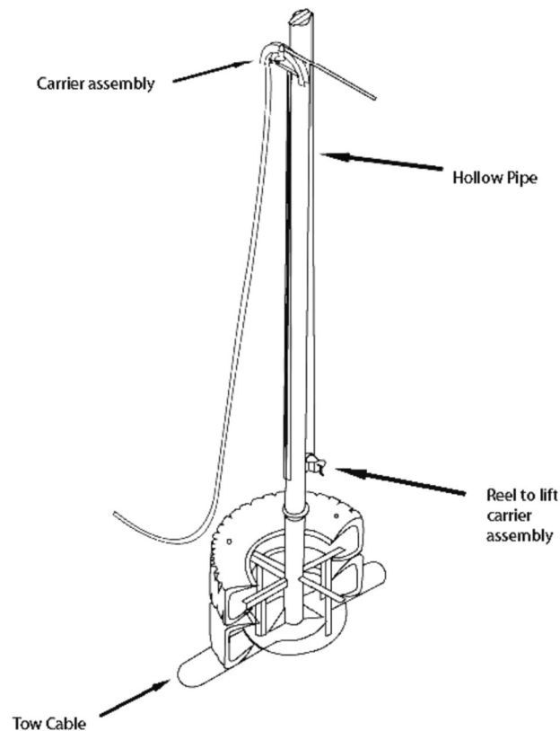
2.18: Cable tower
